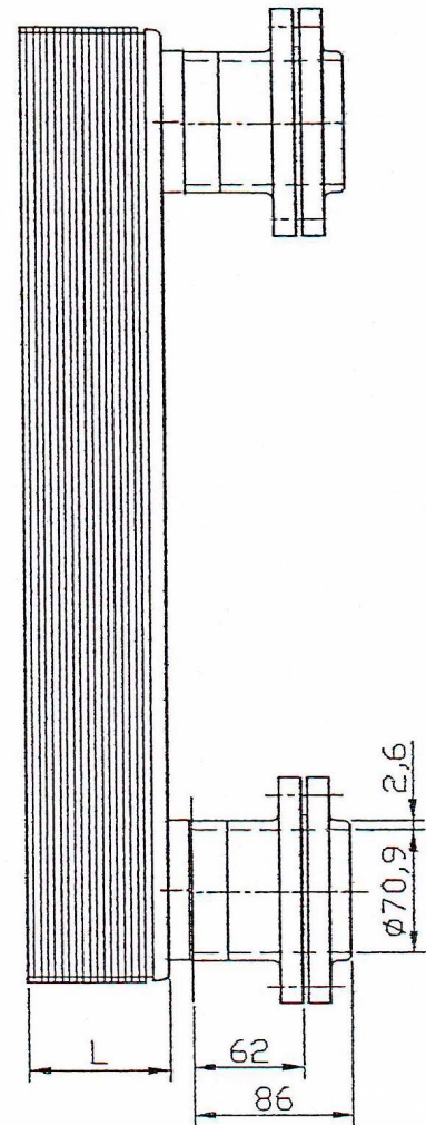
Compac-Flansch DN 65 / PN 40
